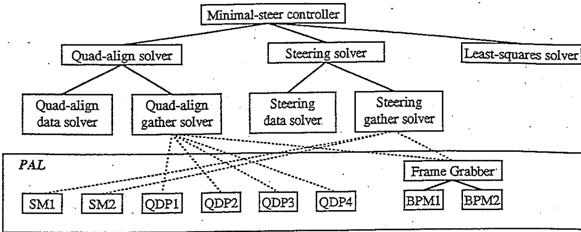
Figure 4. An example of a control hierarchy for minimal quadrupole steering.
